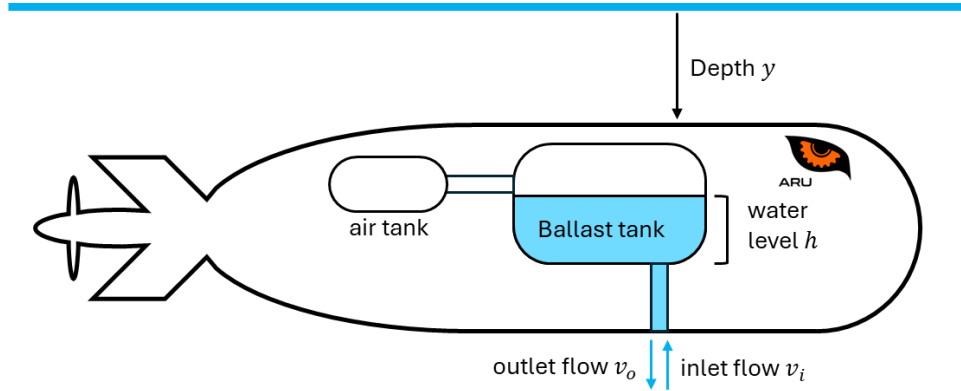
Figure 1: Depth control system in the AUV
